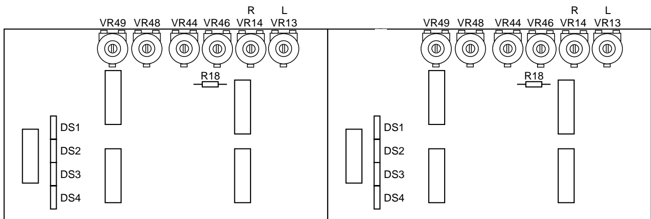
Fig. 26. Simplified component view of Model 12-B signal boards.
