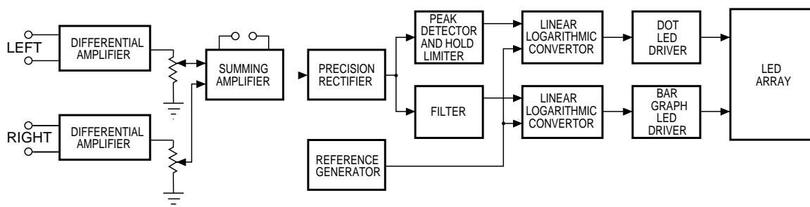
Fig. 25. Block diagram of Model 12-B meter.
