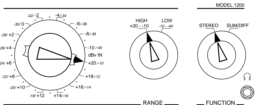
Fig. 7. Initial settings for measuring a stereo signal.
